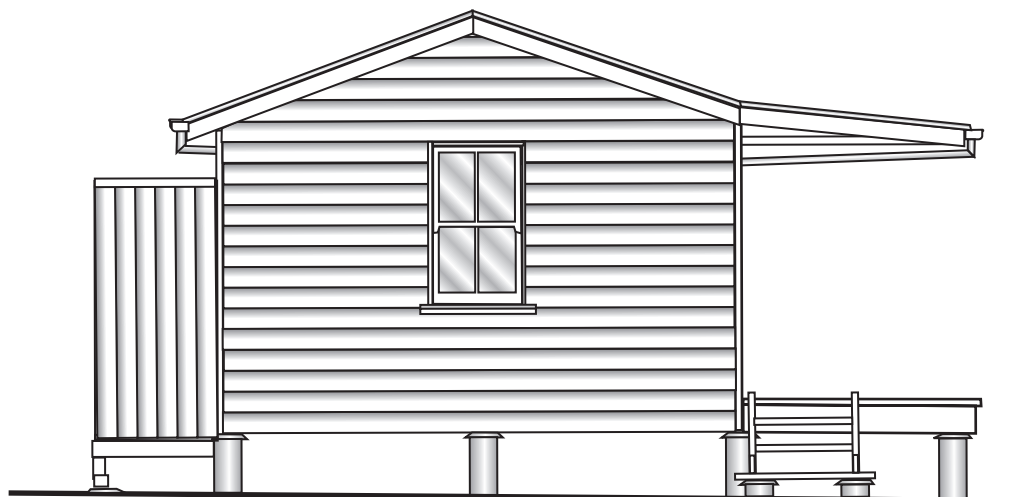
East Elevation
